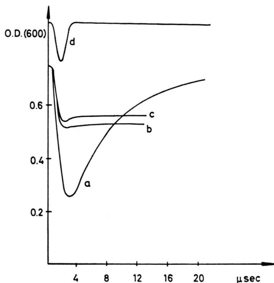
Fig. 2. Magnetic field effect, observed at 600 nm (maximum of thionine ground state absorption), [\text{TH}^\cdot] = 10^{-5} M, solvent methanol, buffered at pH 8.6 (see experimental part). a) Solution without quencher, no influence of magnetic fields between 0 and 4.14 kGauss, b) solution with addition of 2 \times 10^{-3} M p-iodoaniline, zero magnetic field, c) same solution as b), magnetic field 4.14 kGauss, d) profile of the laser flash, arbitrary units.
