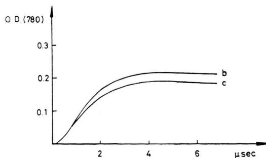
Fig. 3. Magnetic field effect, observed at 780 nm (maximum of thionine semiquinone ( \text{TH}_2^{+\cdot} ) absorption, [\text{TH}^\cdot] = 3 \times 10^{-5} M, 2 \times 10^{-3} M p-iodoaniline, solvent methanol, buffered at pH 8.6, b) at zero magnetic field, c) with magnetic field of 4.14 kGauss.
